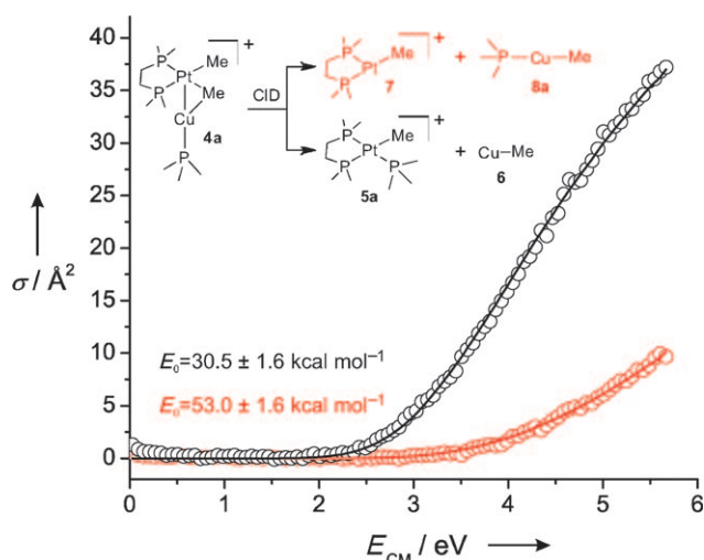
Figure 3. Zero-pressure extrapolated cross-sections (circles) and L-CID fitted curves (lines) as a function of center-of-mass energy for the two competing CID reactions of ion 4a .
